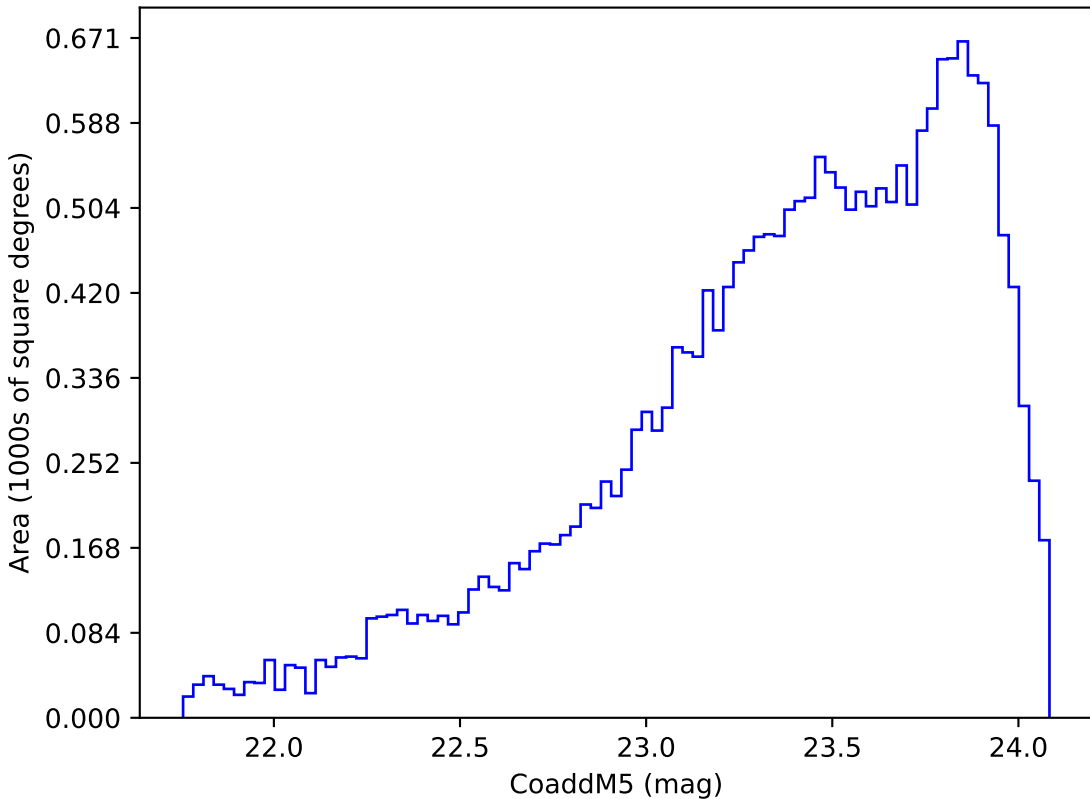
too_elab_r8_d2_giz_v3.4_10yrs Yr 3-4 y band: CoaddM5
