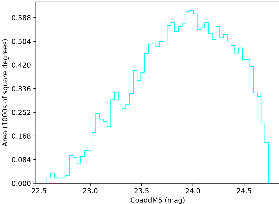
too_elab_r8_d2_giz_v3.4_10yrs Yr 3-4 u band: CoaddM5
