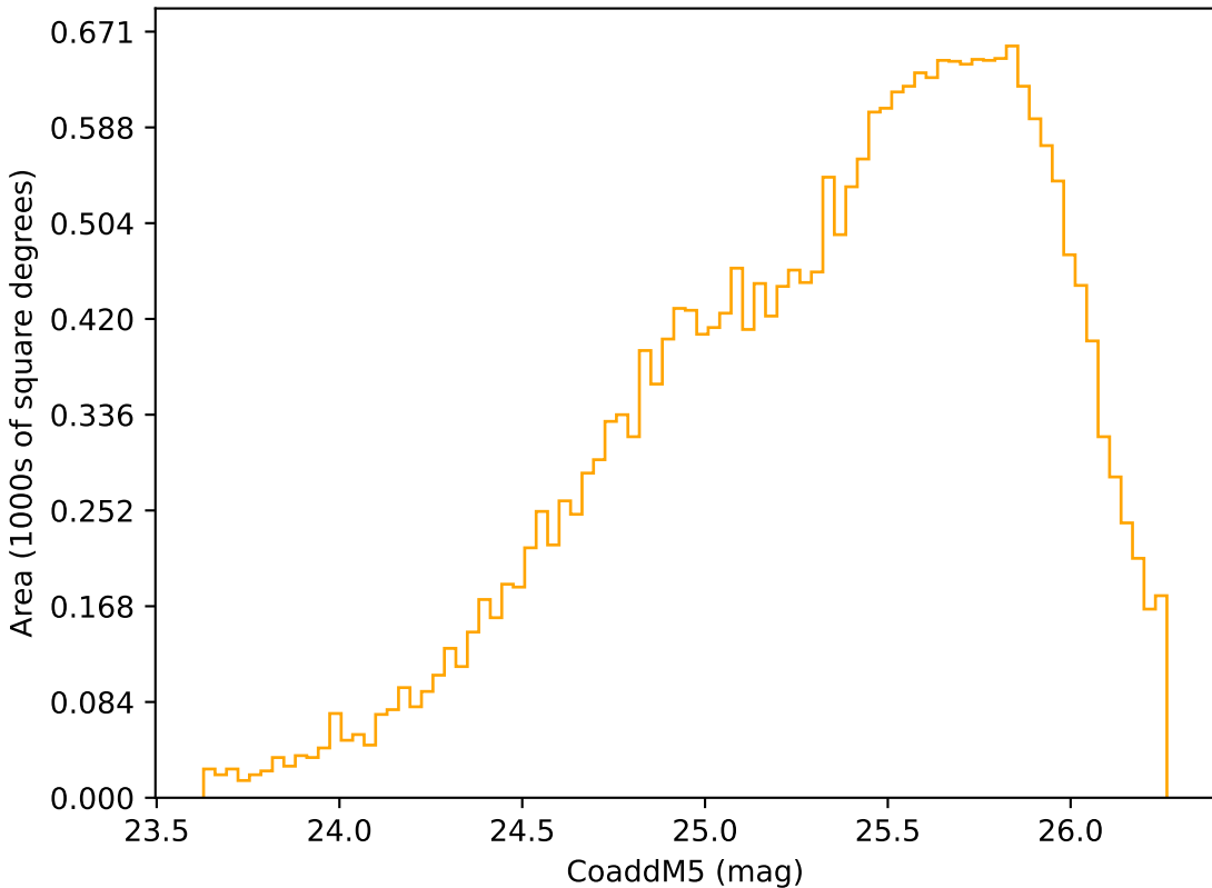
too_elab_r8_d2_giz_v3.4_10yrs Yr 3-4 r band: CoaddM5
