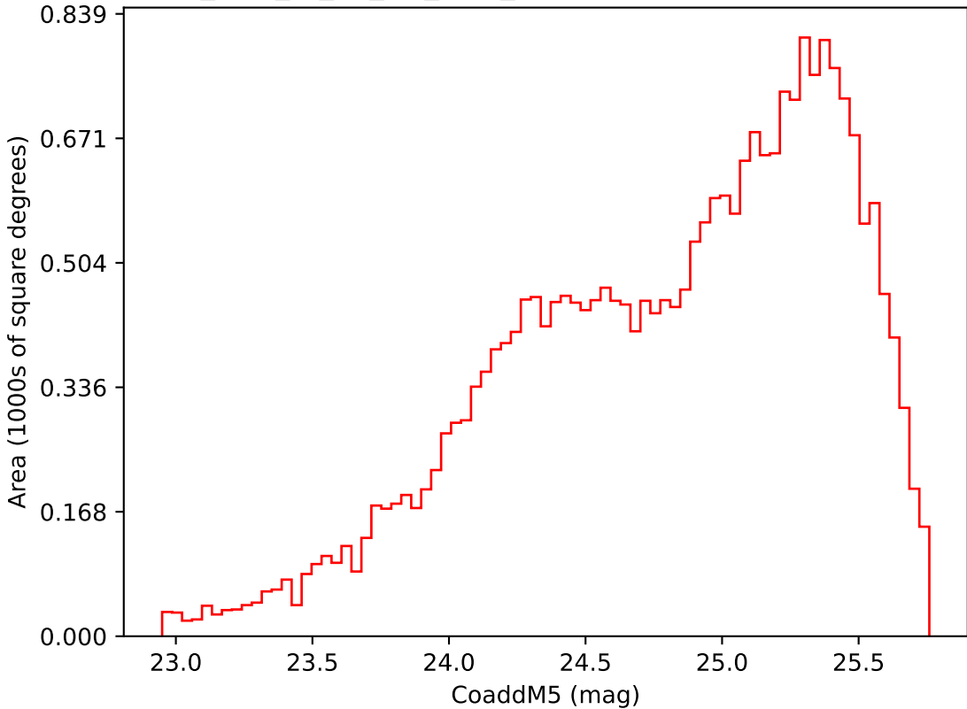
too_elab_r8_d2_giz_v3.4_10yrs Yr 3-4 i band: CoaddM5
