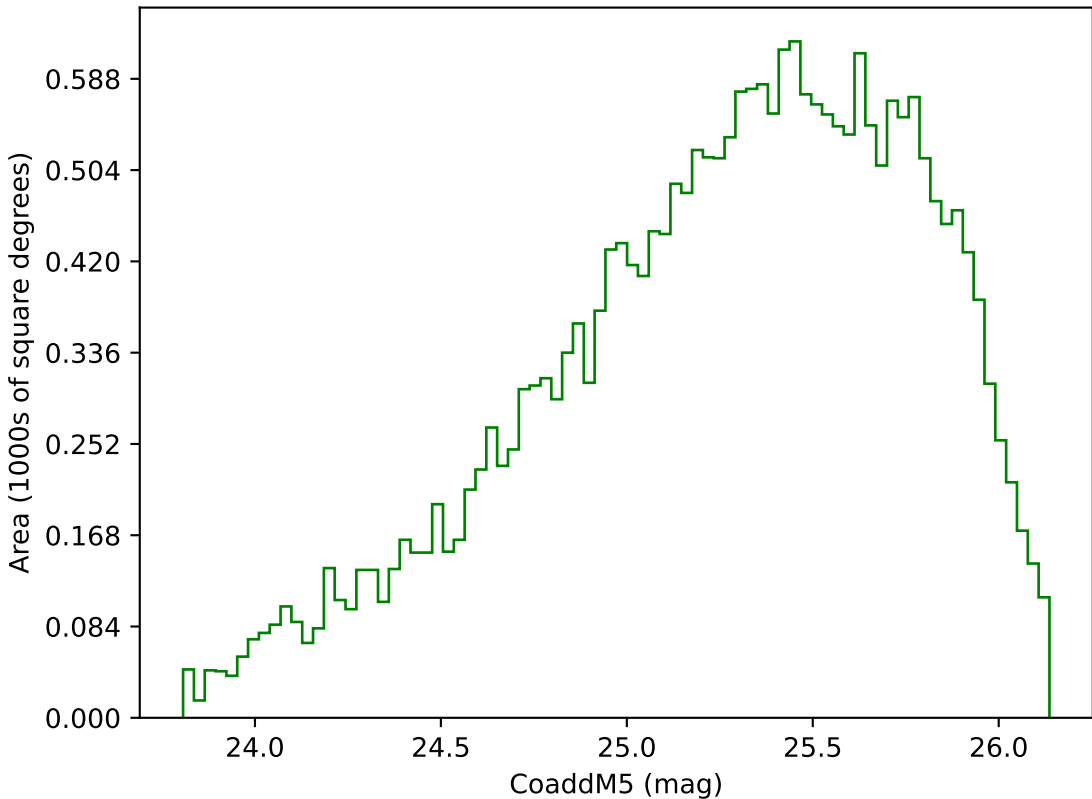
too_elab_r8_d2_giz_v3.4_10yrs Yr 3-4 g band: CoaddM5
