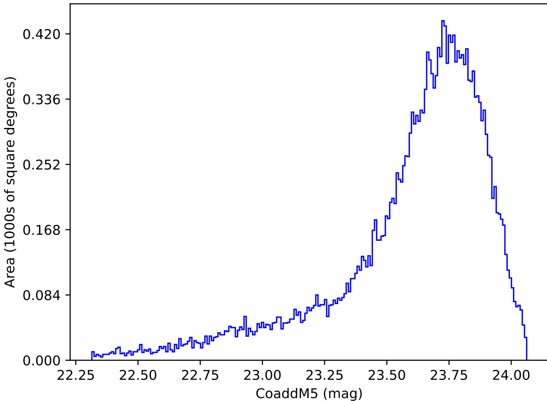
too_elab_r8_d2_giz_v3.4_10yrs Yr 1 y band: CoaddM5
