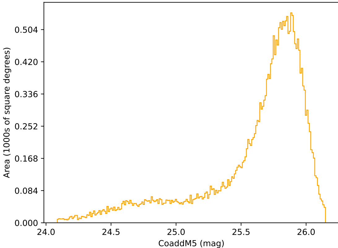
too_elab_r8_d2_giz_v3.4_10yrs Yr 1 r band: CoaddM5
