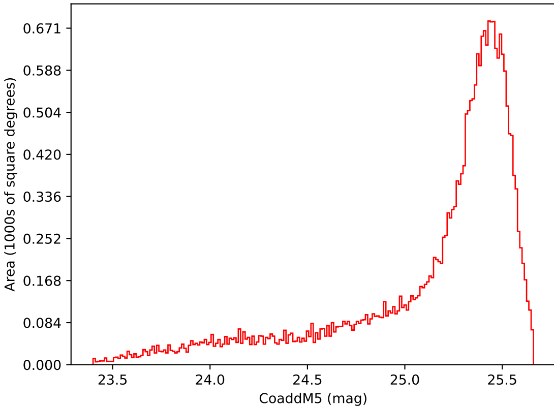
too_elab_r8_d2_giz_v3.4_10yrs Yr 1 i band: CoaddM5
