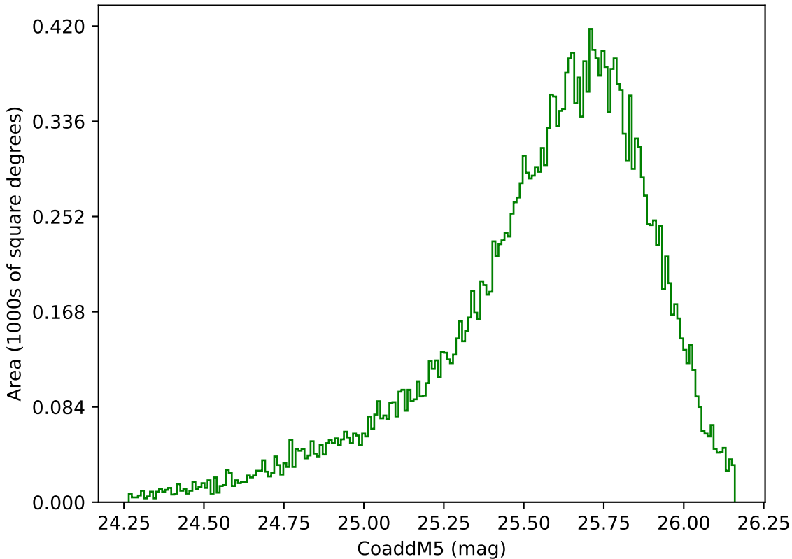
too_elab_r8_d2_giz_v3.4_10yrs Yr 1 g band: CoaddM5
