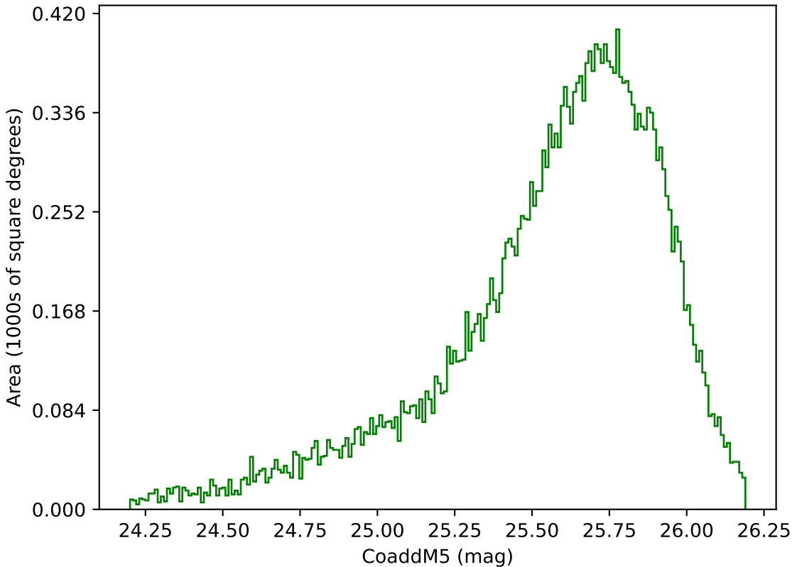
too_elab_r8_d2_giz_v3.4_10yrs Yr 1 g band: CoaddM5
