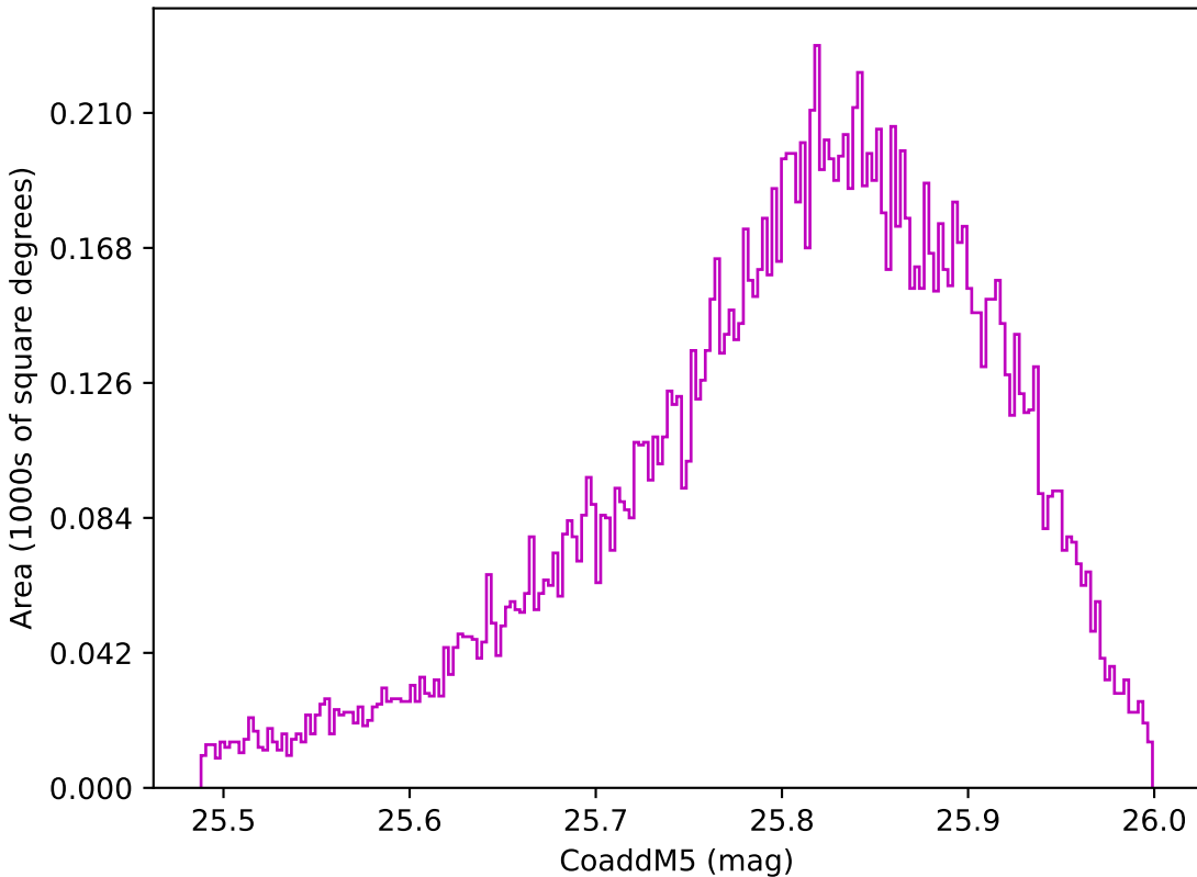
too_elab_r8_d2_giz_v3.4_10yrs WFD z band: CoaddM5
