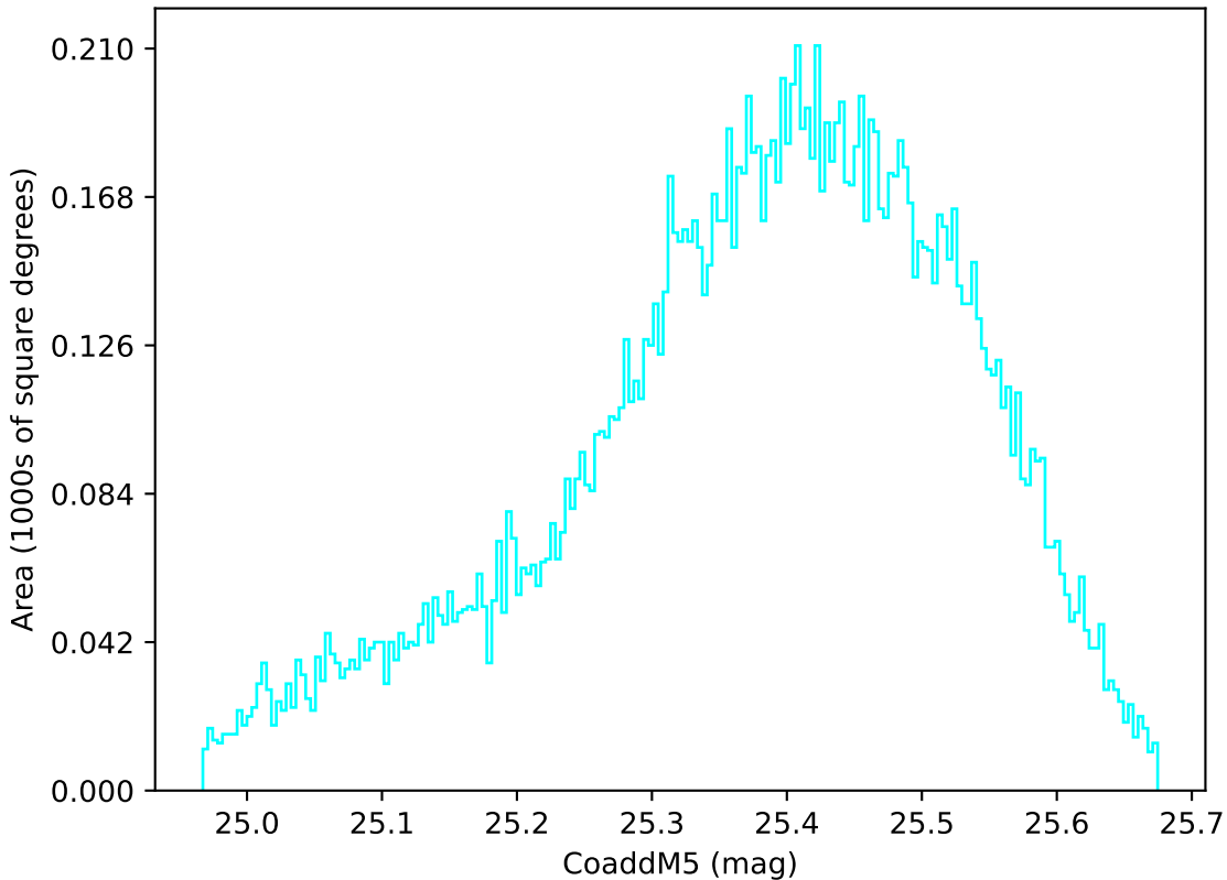
too_elab_r8_d2_giz_v3.4_10yrs WFD u band: CoaddM5
