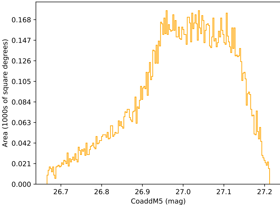
too_elab_r8_d2_giz_v3.4_10yrs WFD r band: CoaddM5
