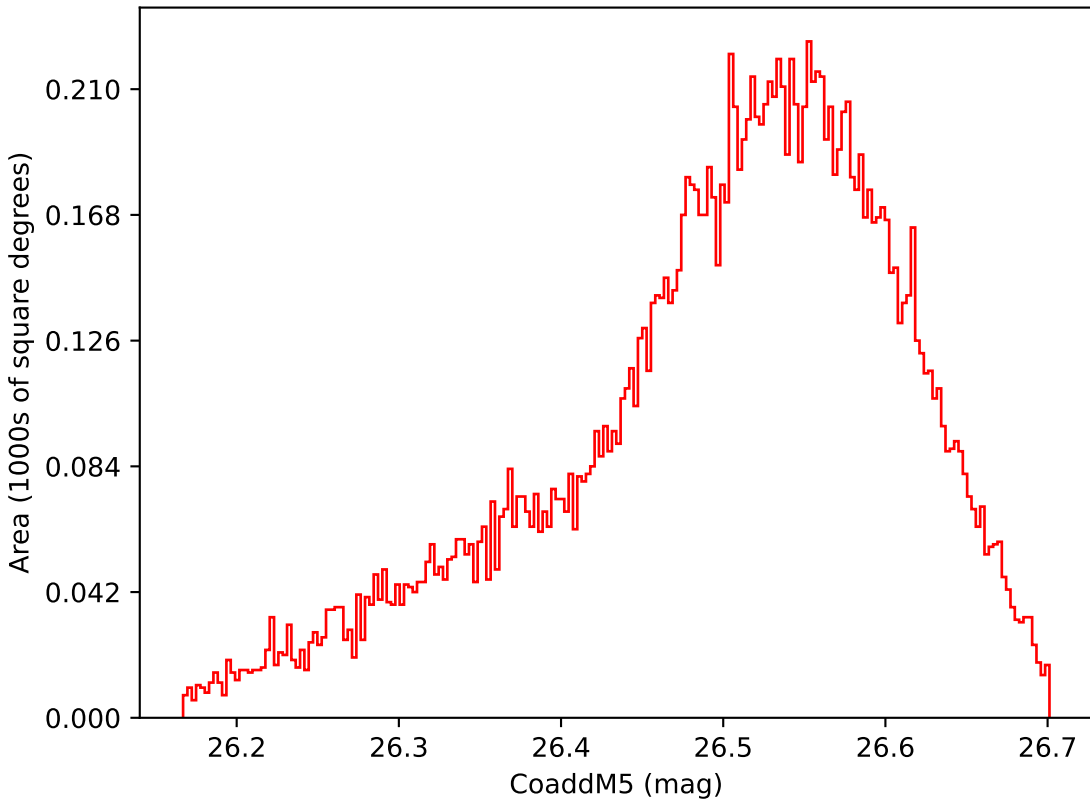
too_elab_r8_d2_giz_v3.4_10yrs WFD i band: CoaddM5
