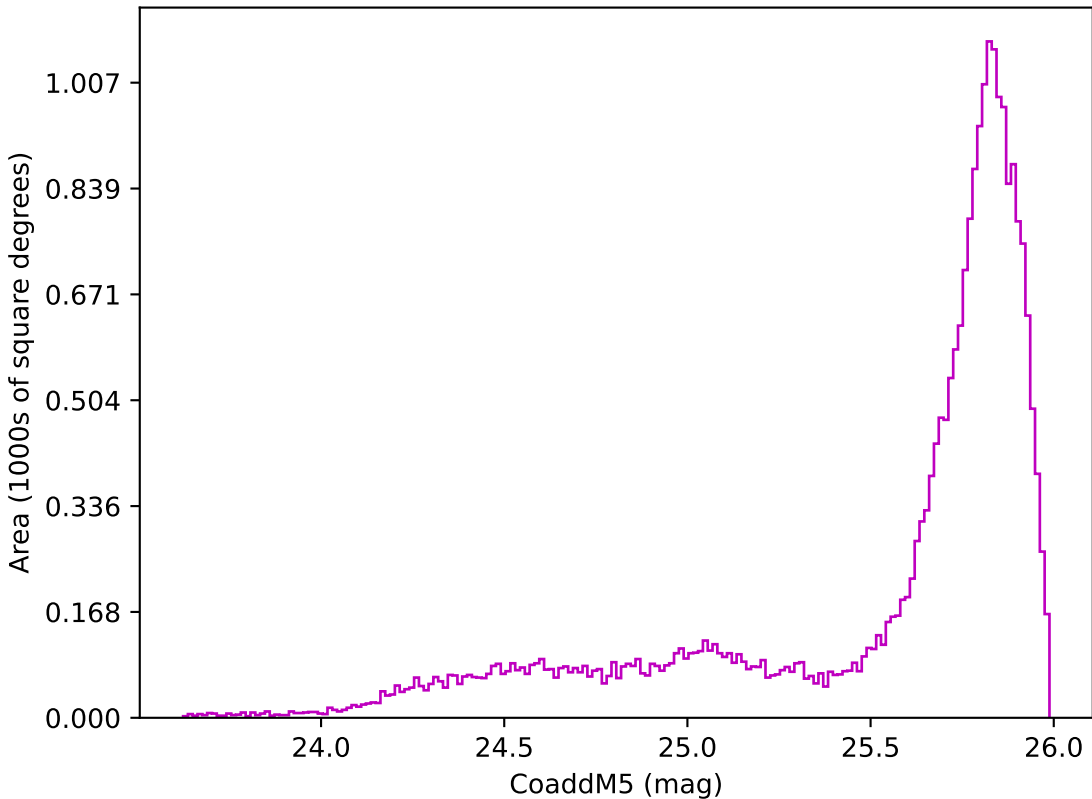
too_elab_r8_d2_giz_v3.4_10yrs All sky z band: CoaddM5
