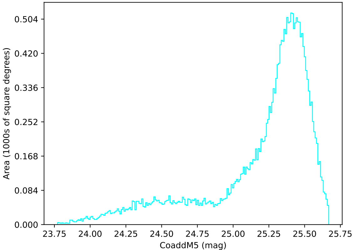
too_elab_r8_d2_giz_v3.4_10yrs All sky u band: CoaddM5
