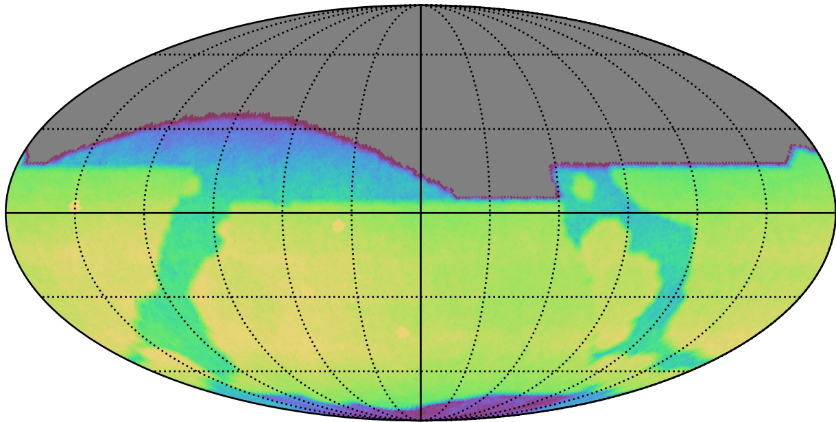
too_elab_r8_d2_giz_v3.4_10yrs All sky r band: CoaddM5
