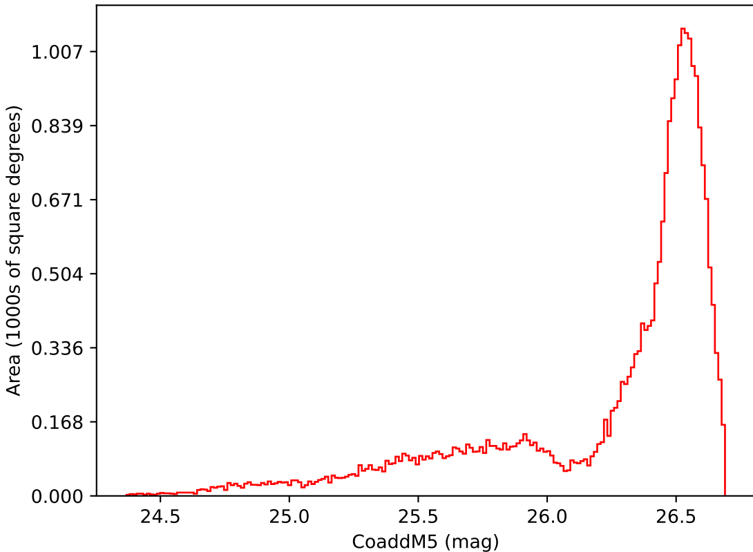
too_elab_r8_d2_giz_v3.4_10yrs All sky i band: CoaddM5
