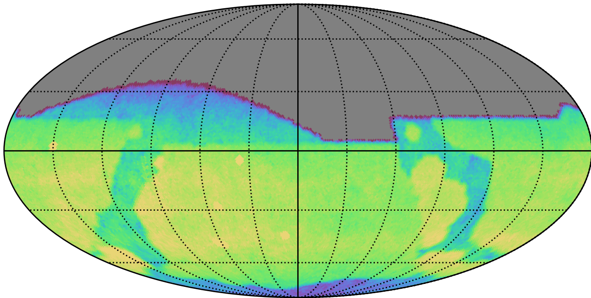
too_elab_r8_d2_giz_v3.4_10yrs All sky g band: CoaddM5
