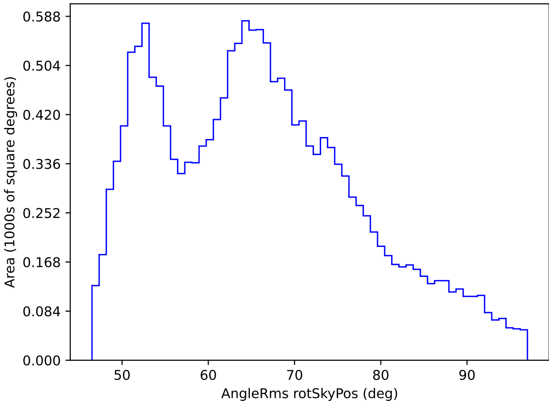
too_elab_r8_d2_giz_v3.4_10yrs WFD r band: AngleRms rotSkyPos
