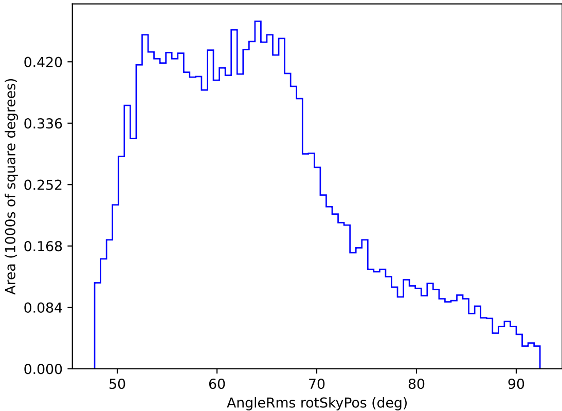
too_elab_r8_d2_giz_v3.4_10yrs WFD i band: AngleRms rotSkyPos
