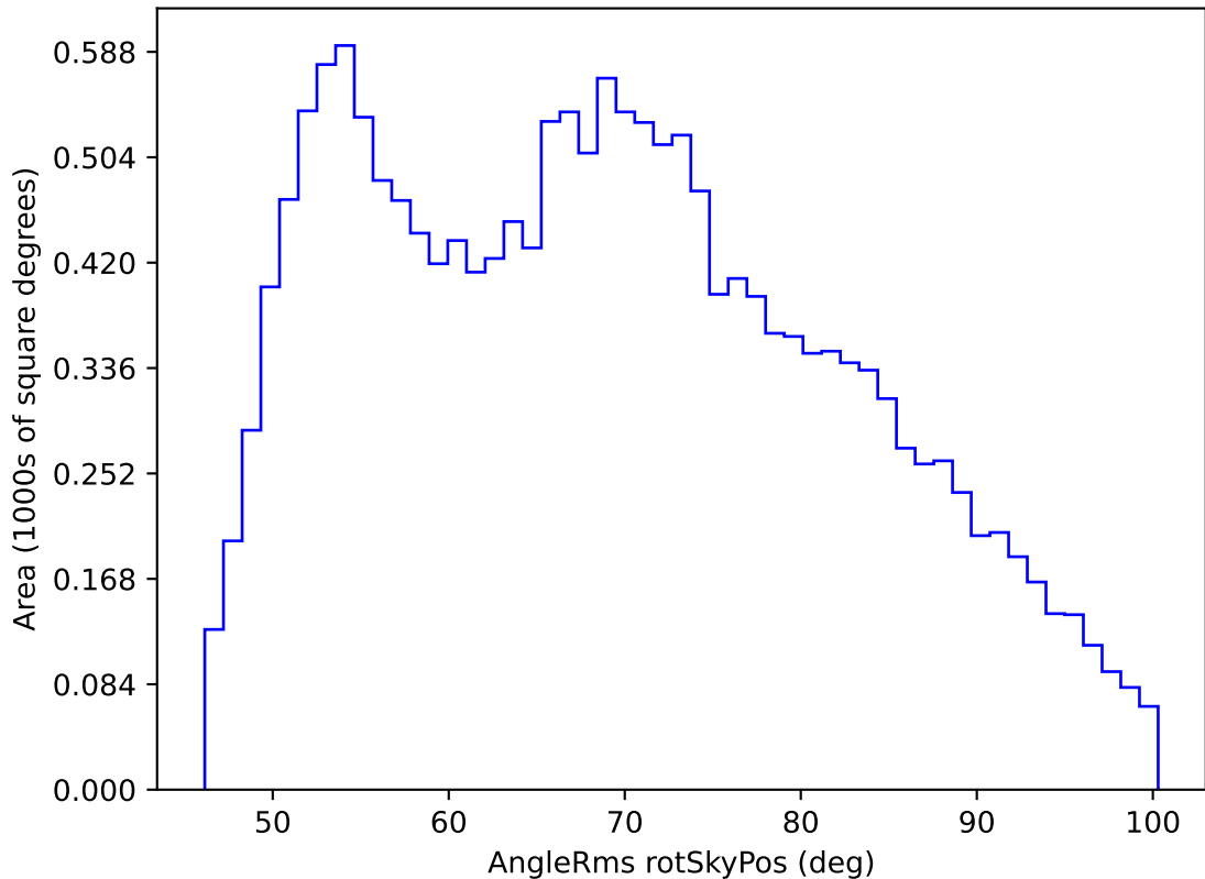
too_elab_r8_d2_giz_v3.4_10yrs WFD g band: AngleRms rotSkyPos
