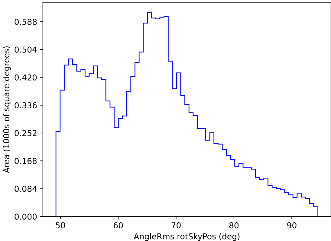
too_elab_r8_d2_giz_v3.4_10yrs WFD all bands: AngleRms rotSkyPos
