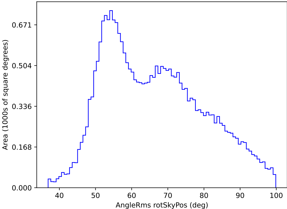
too_elab_r8_d2_giz_v3.4_10yrs All sky g band: AngleRms rotSkyPos
