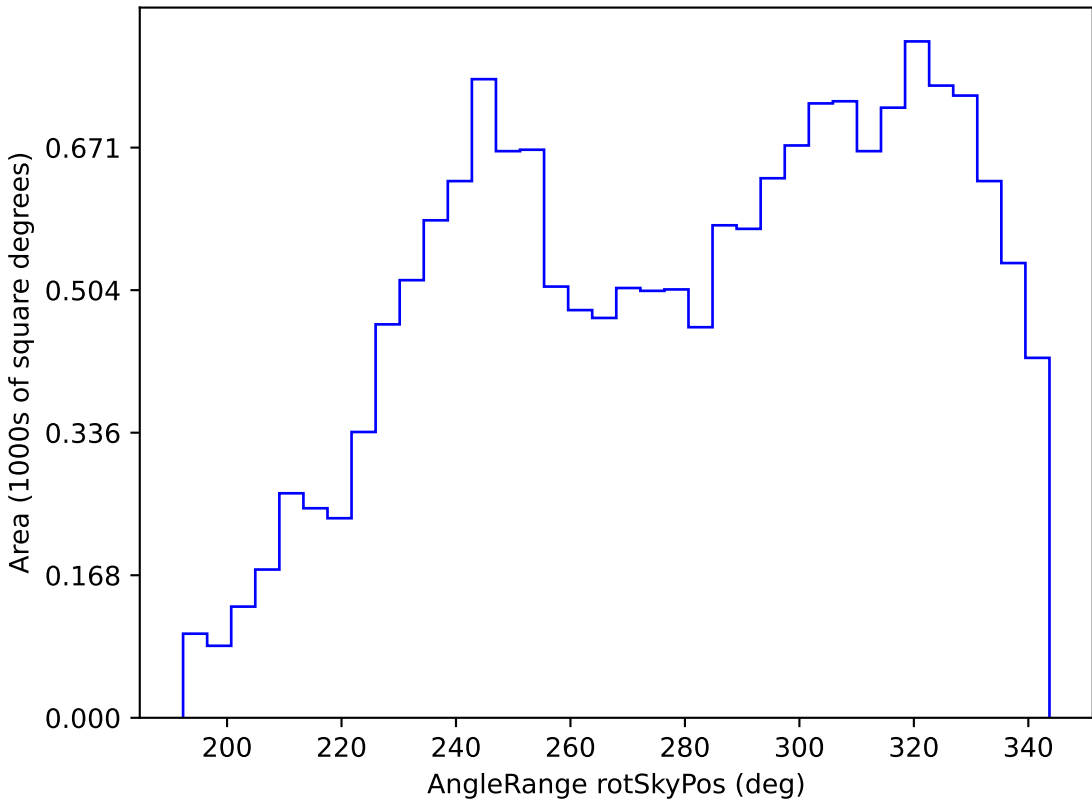
too_elab_r8_d2_giz_v3.4_10yrs WFD z band: AngleRange rotSkyPos
