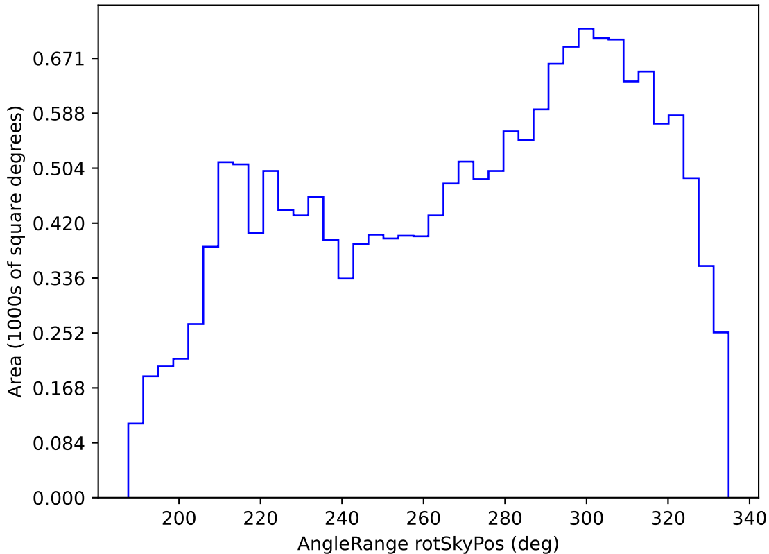
too_elab_r8_d2_giz_v3.4_10yrs WFD g band: AngleRange rotSkyPos
