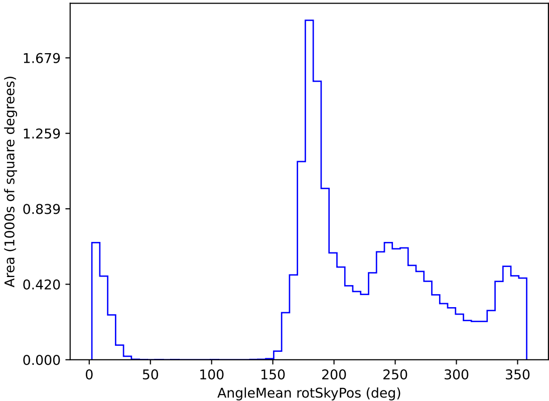
too_elab_r8_d2_giz_v3.4_10yrs WFD y band: AngleMean rotSkyPos
