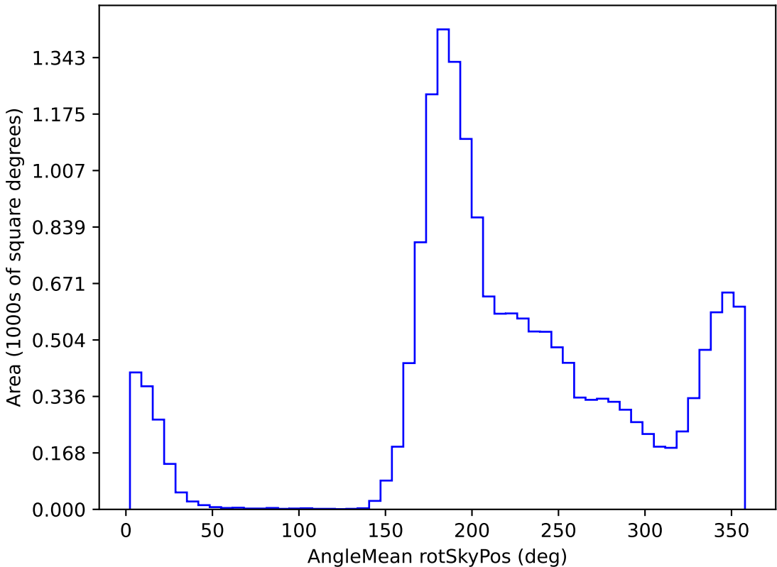
too_elab_r8_d2_giz_v3.4_10yrs WFD u band: AngleMean rotSkyPos
