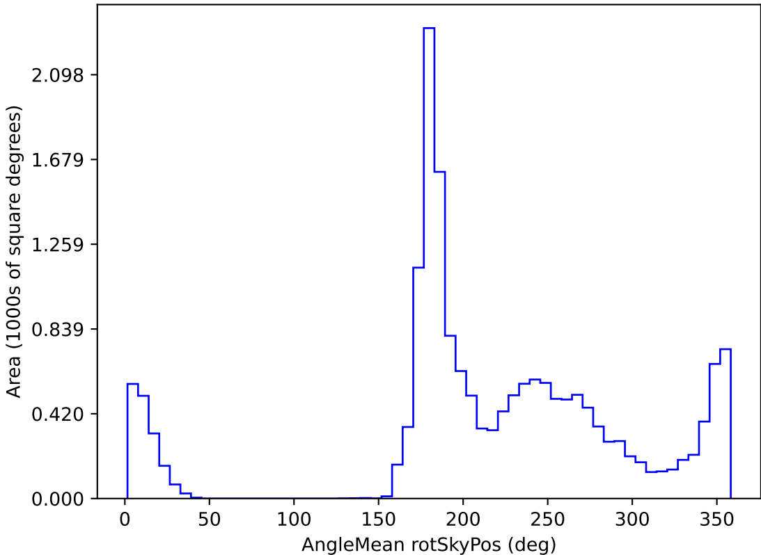
too_elab_r8_d2_giz_v3.4_10yrs WFD i band: AngleMean rotSkyPos
