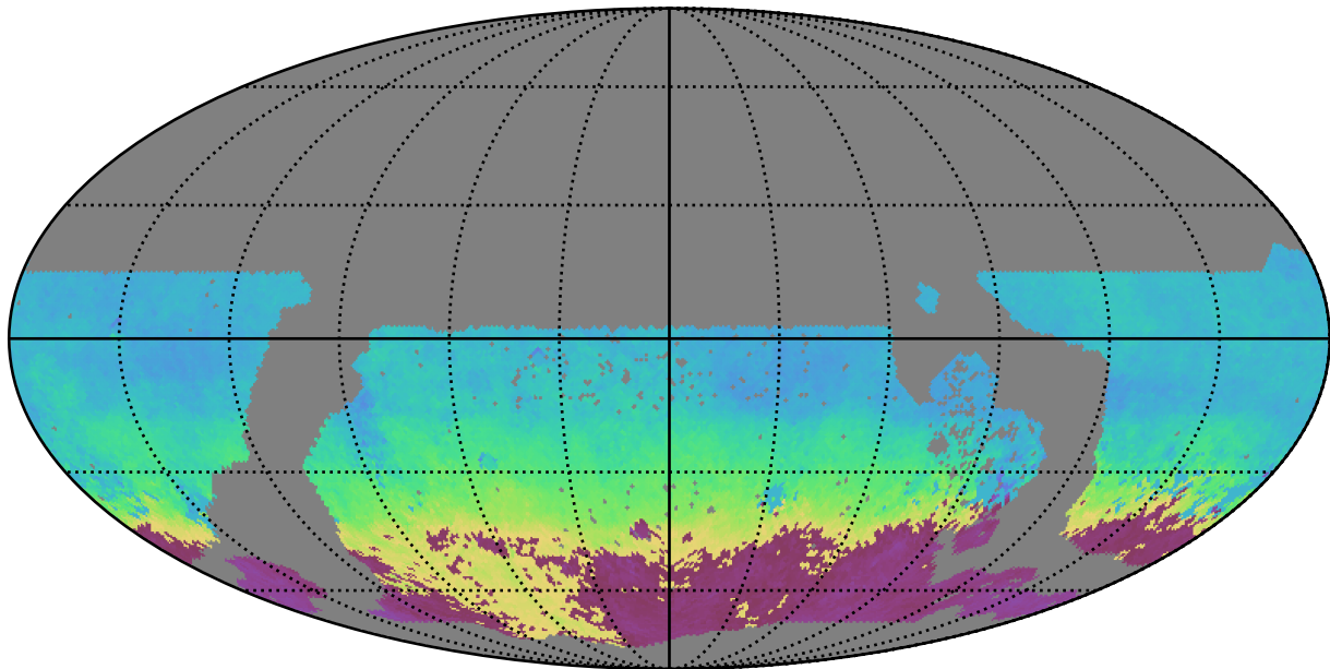
too_elab_r8_d2_giz_v3.4_10yrs WFD g band: AngleMean rotSkyPos
