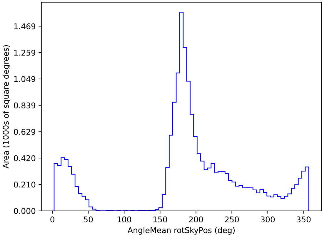
too_elab_r8_d2_giz_v3.4_10yrs WFD g band: AngleMean rotSkyPos
