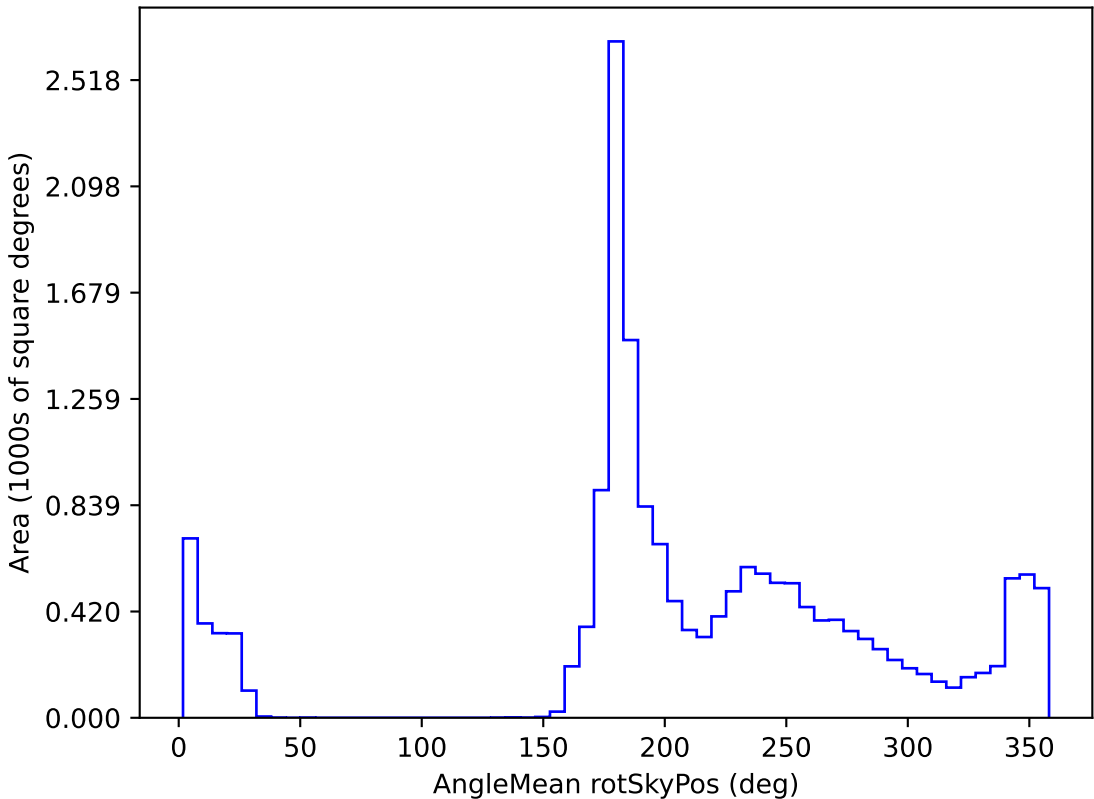
too_elab_r8_d2_giz_v3.4_10yrs WFD all bands: AngleMean rotSkyPos
