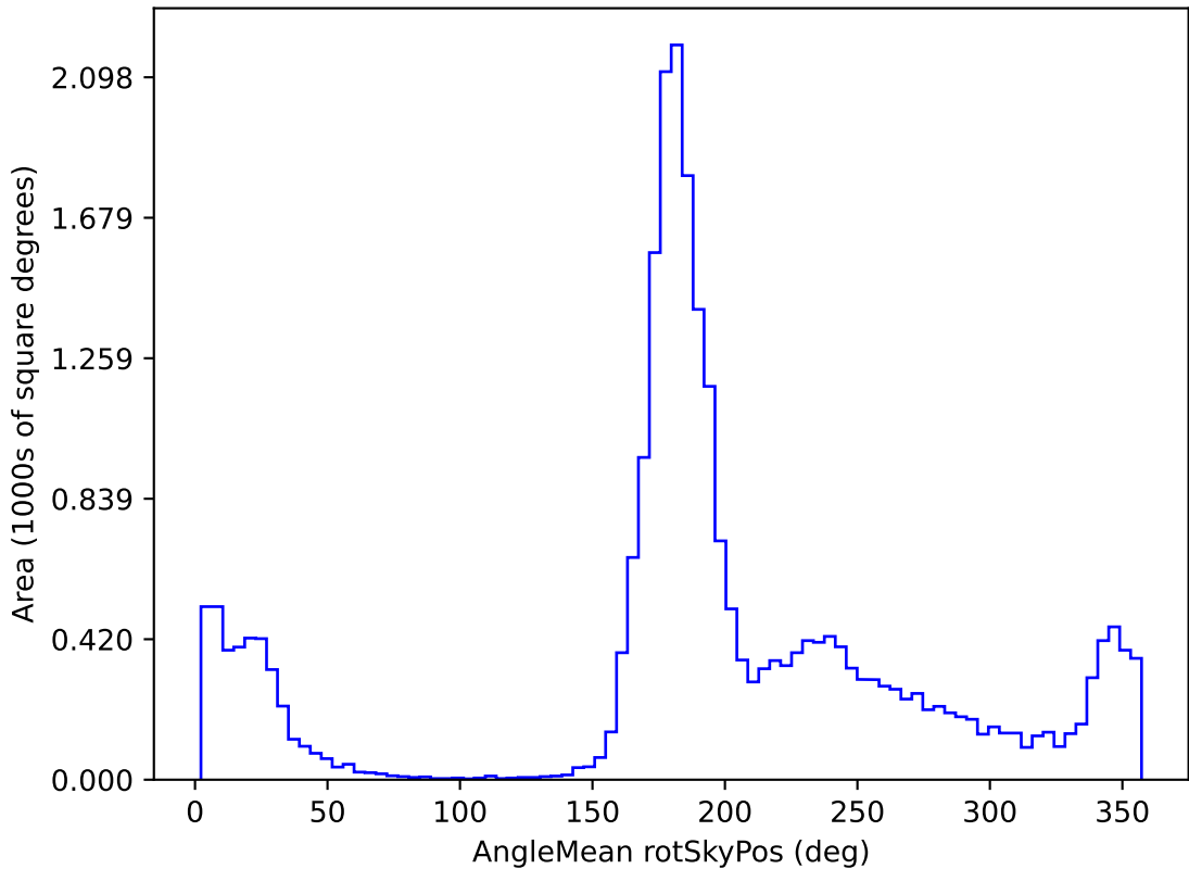
too_elab_r8_d2_giz_v3.4_10yrs All sky r band: AngleMean rotSkyPos
