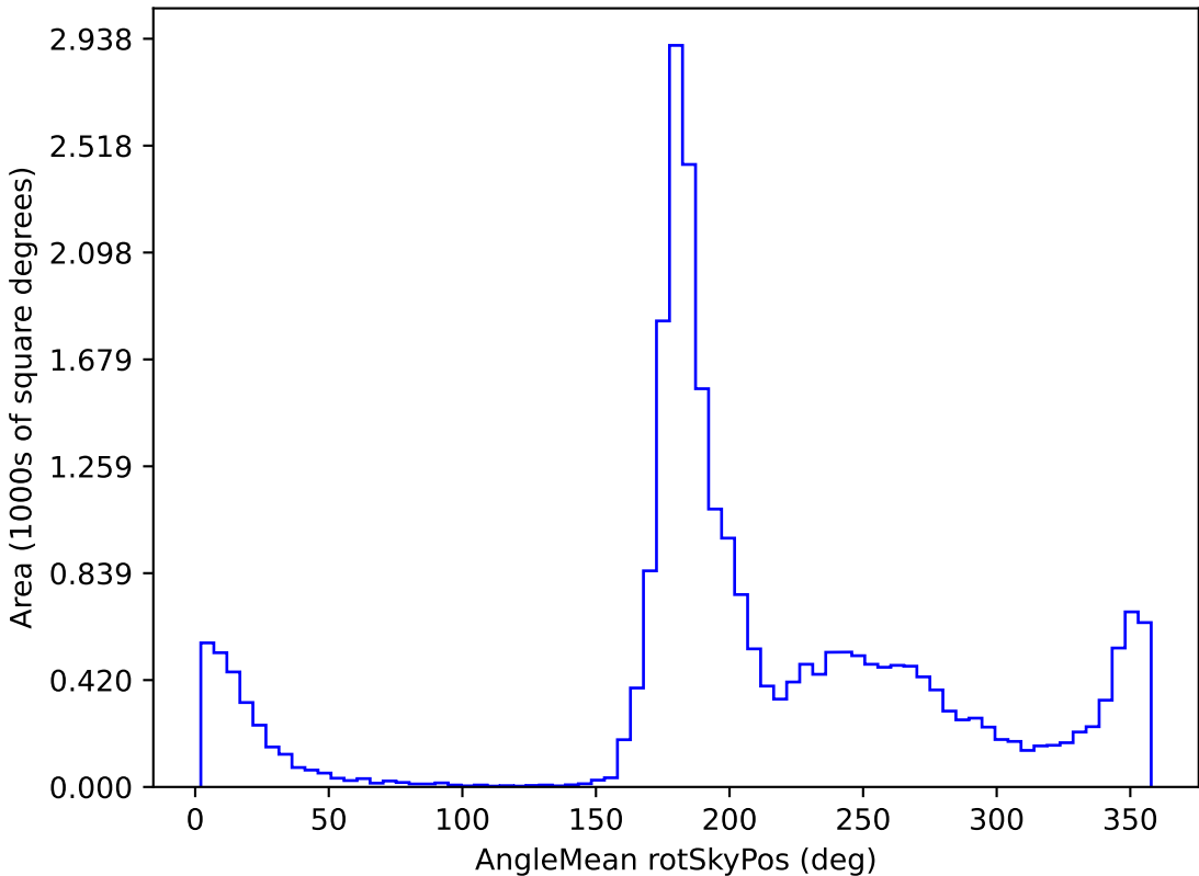
too_elab_r8_d2_giz_v3.4_10yrs All sky i band: AngleMean rotSkyPos
