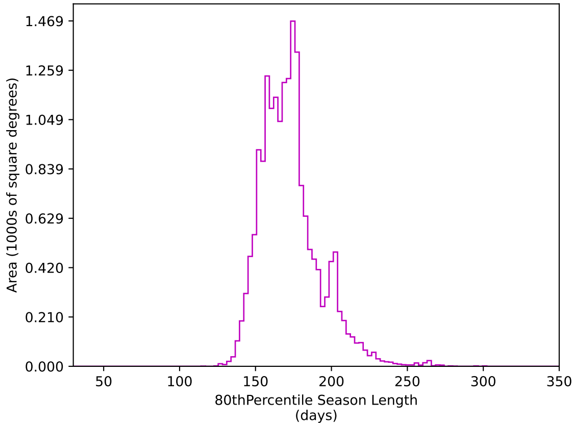
too_elab_r8_d2_giz_v3.4_10yrs WFD z band: 80thPercentile Season Length
