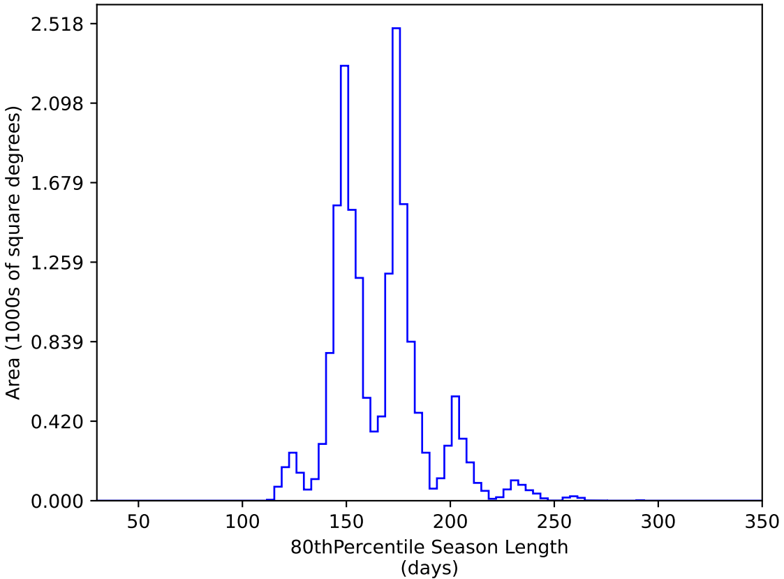
too_elab_r8_d2_giz_v3.4_10yrs WFD y band: 80thPercentile Season Length
