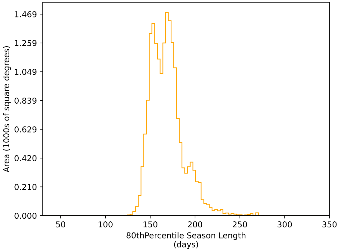
too_elab_r8_d2_giz_v3.4_10yrs WFD r band: 80thPercentile Season Length
