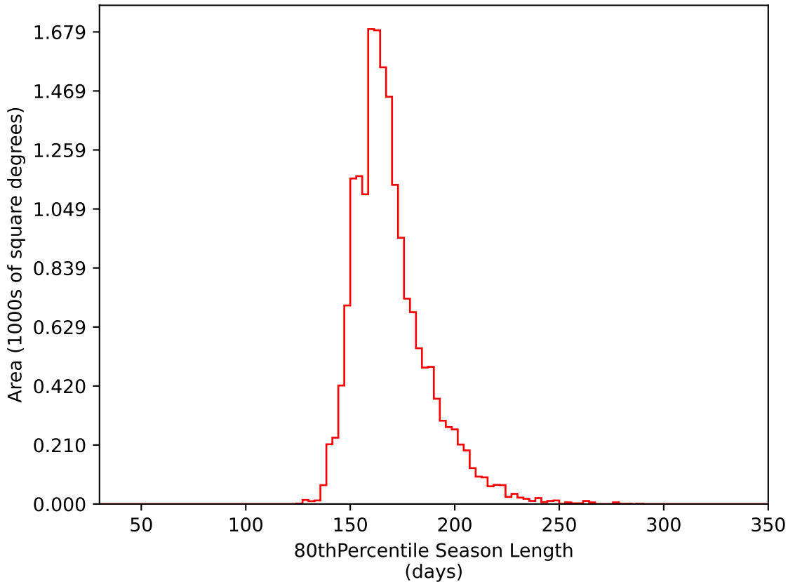
too_elab_r8_d2_giz_v3.4_10yrs WFD i band: 80thPercentile Season Length
