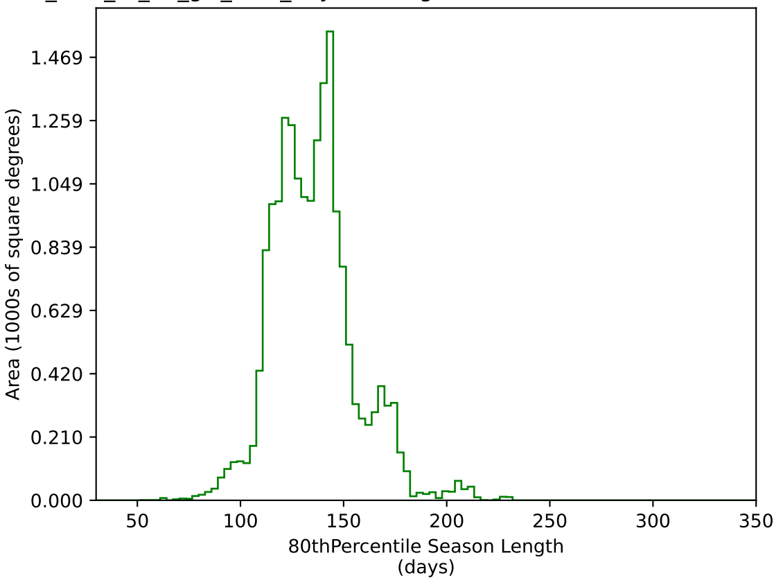
too_elab_r8_d2_giz_v3.4_10yrs WFD g band: 80thPercentile Season Length
