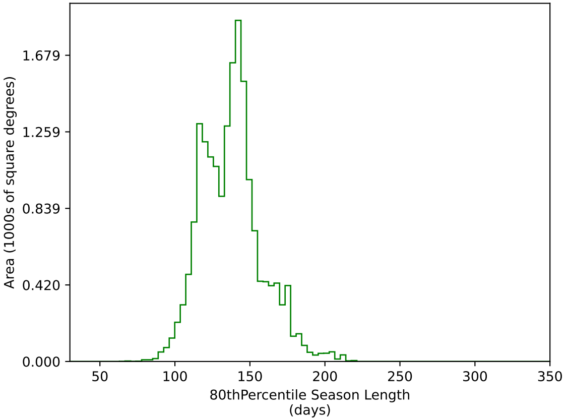
too_elab_r8_d2_giz_v3.4_10yrs WFD g band: 80thPercentile Season Length
