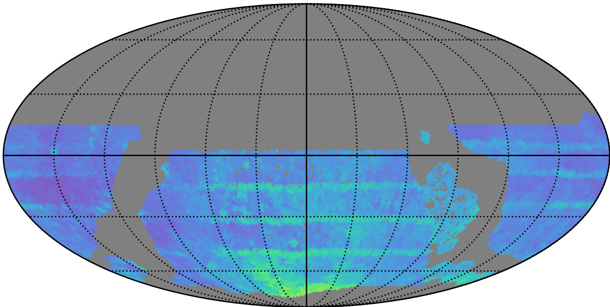
too_elab_r8_d2_giz_v3.4_10yrs WFD all bands: 80thPercentile Season Length
