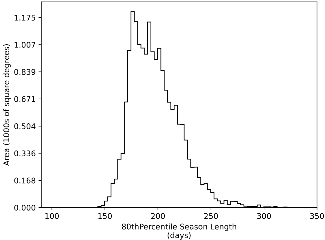
too_elab_r8_d2_giz_v3.4_10yrs WFD all bands: 80thPercentile Season Length
