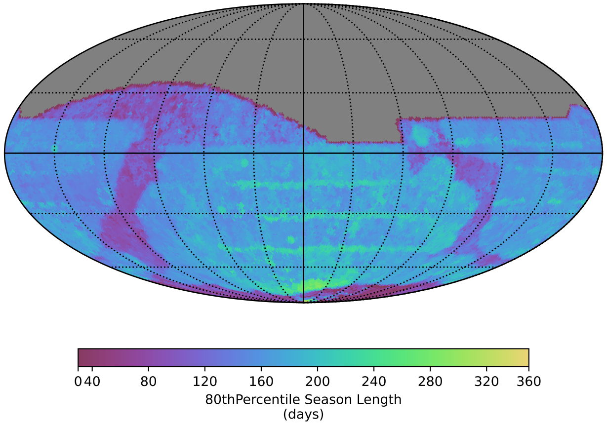
too_elab_r8_d2_giz_v3.4_10yrs All sky z band: 80thPercentile Season Length
