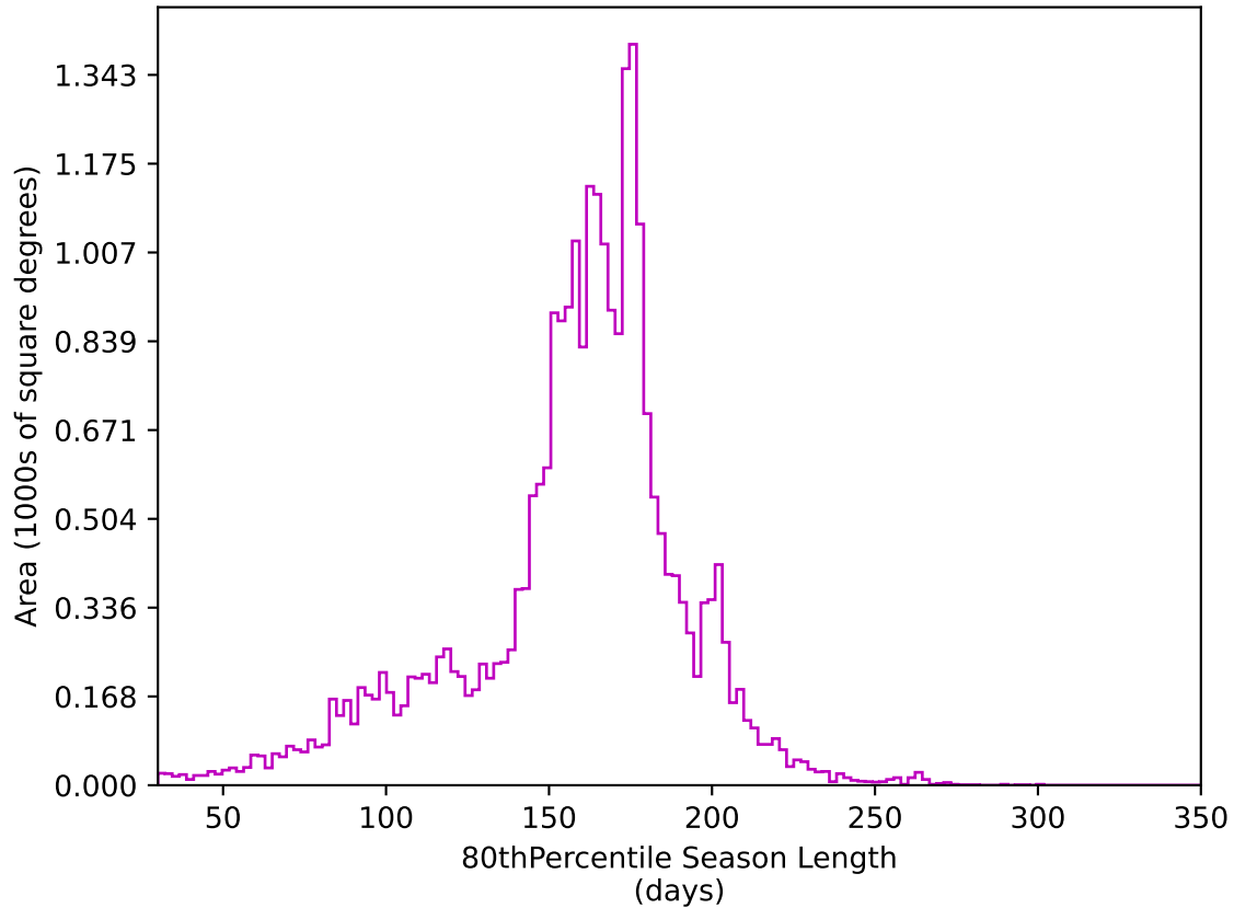
too_elab_r8_d2_giz_v3.4_10yrs All sky z band: 80thPercentile Season Length
