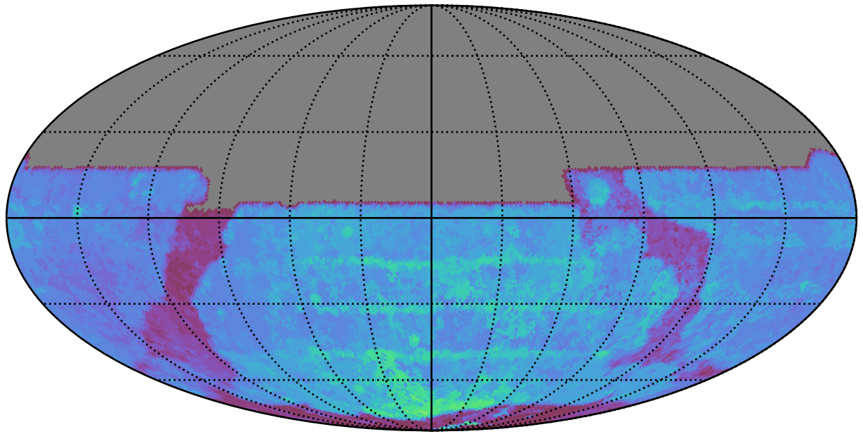
too_elab_r8_d2_giz_v3.4_10yrs All sky y band: 80thPercentile Season Length
