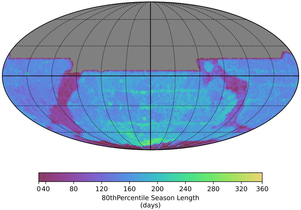
too_elab_r8_d2_giz_v3.4_10yrs All sky y band: 80thPercentile Season Length
