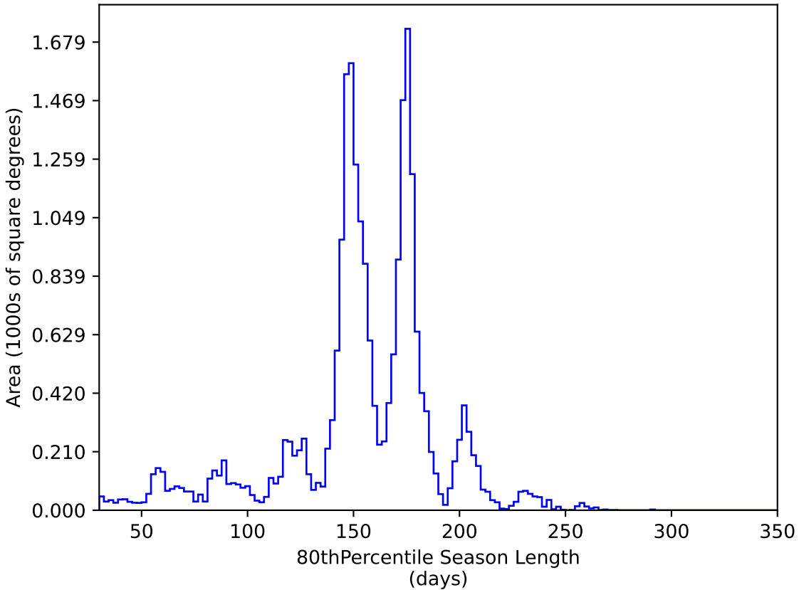
too_elab_r8_d2_giz_v3.4_10yrs All sky y band: 80thPercentile Season Length
