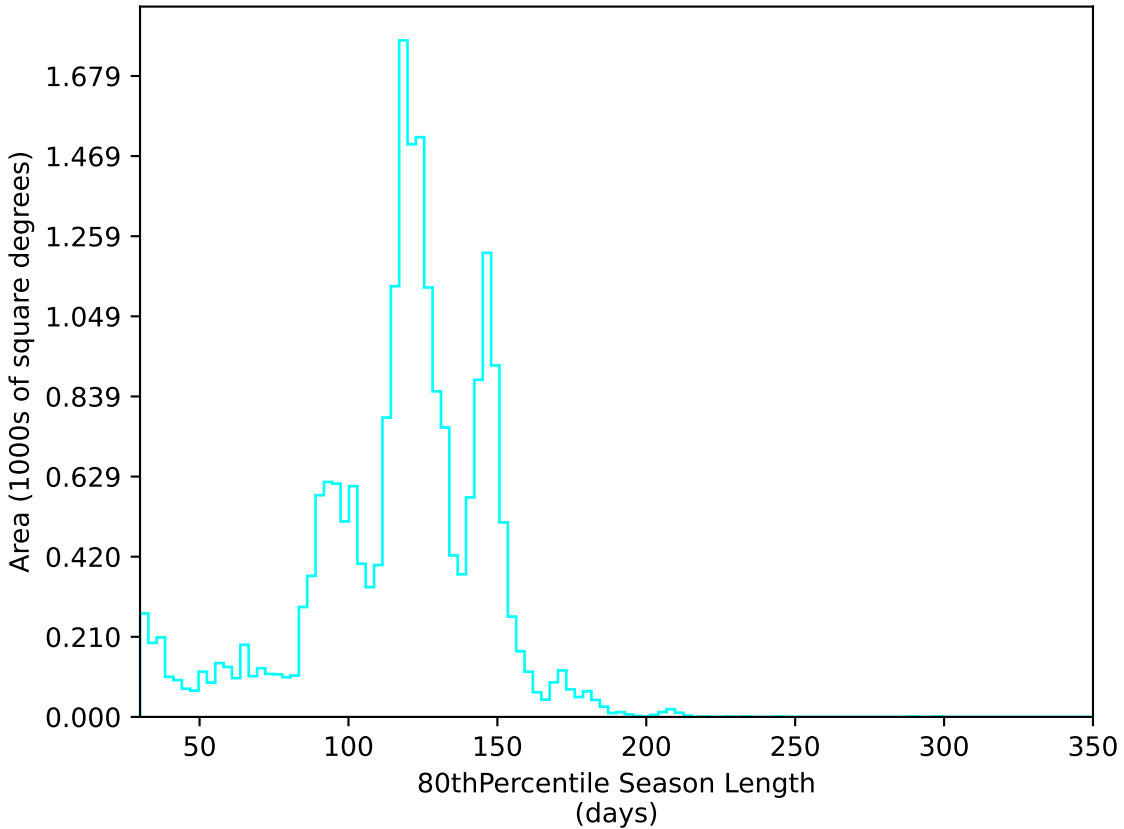
too_elab_r8_d2_giz_v3.4_10yrs All sky u band: 80thPercentile Season Length
