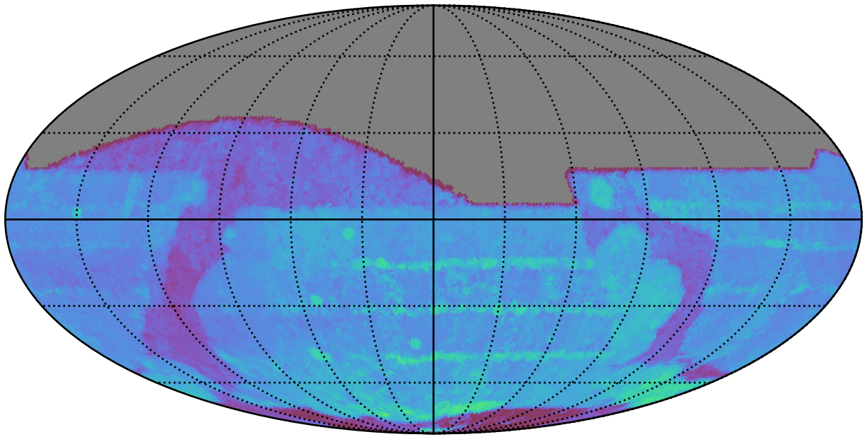
too_elab_r8_d2_giz_v3.4_10yrs All sky r band: 80thPercentile Season Length
