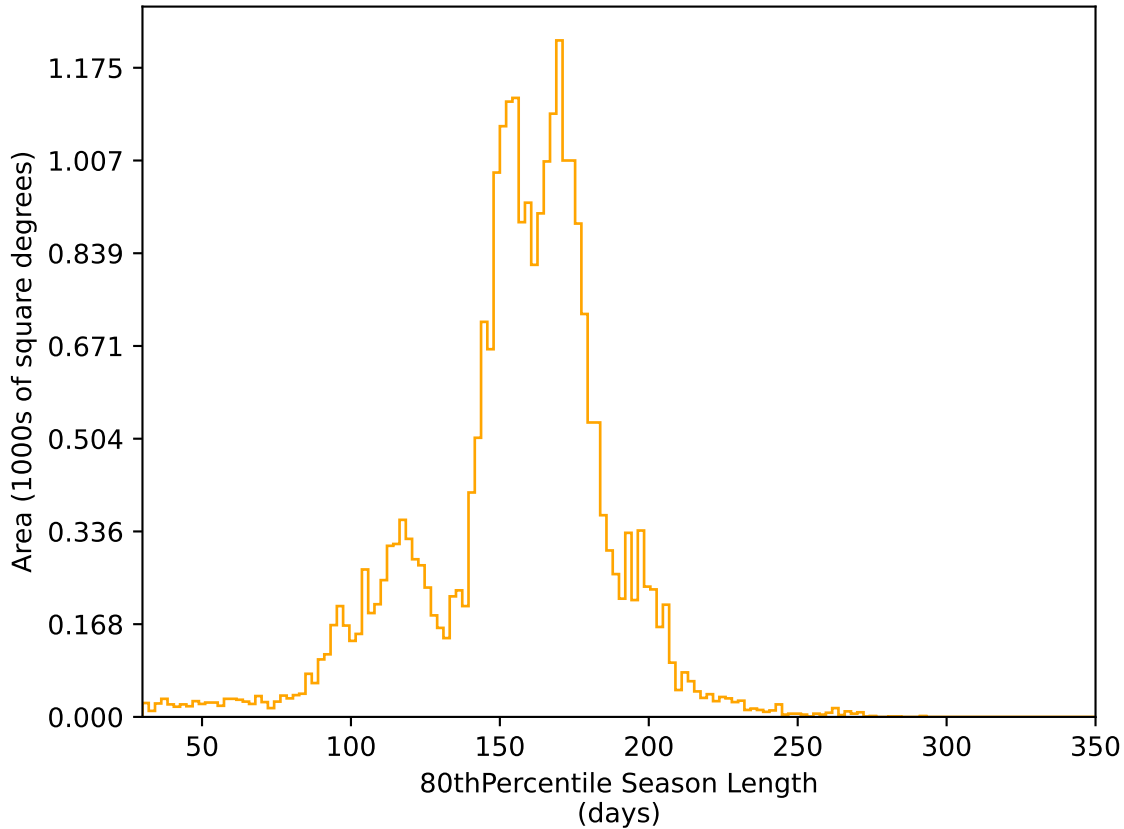
too_elab_r8_d2_giz_v3.4_10yrs All sky r band: 80thPercentile Season Length
