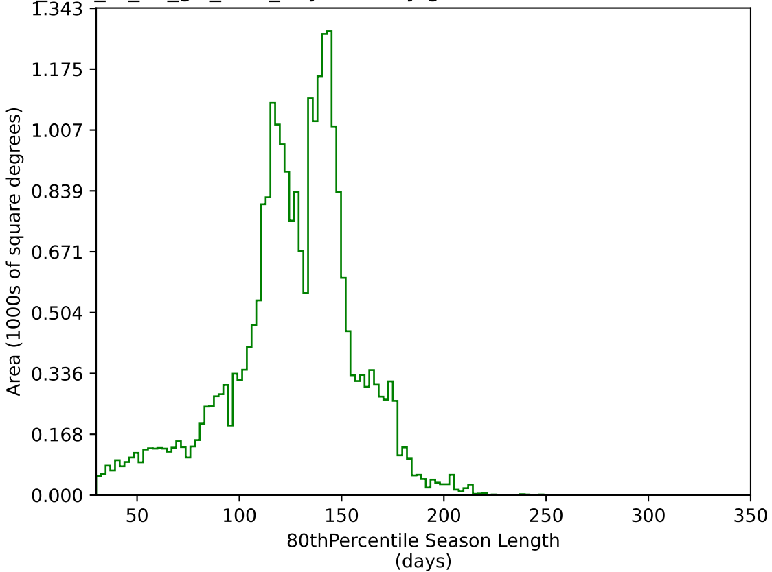
too_elab_r8_d2_giz_v3.4_10yrs All sky g band: 80thPercentile Season Length
