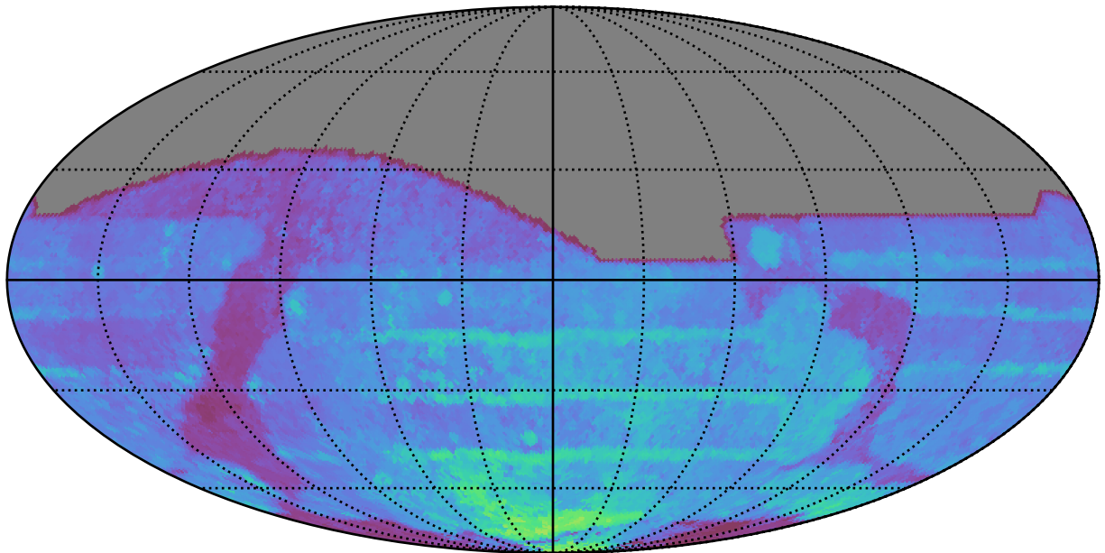
too_elab_r8_d2_giz_v3.4_10yrs All sky all bands: 80thPercentile Season Length
