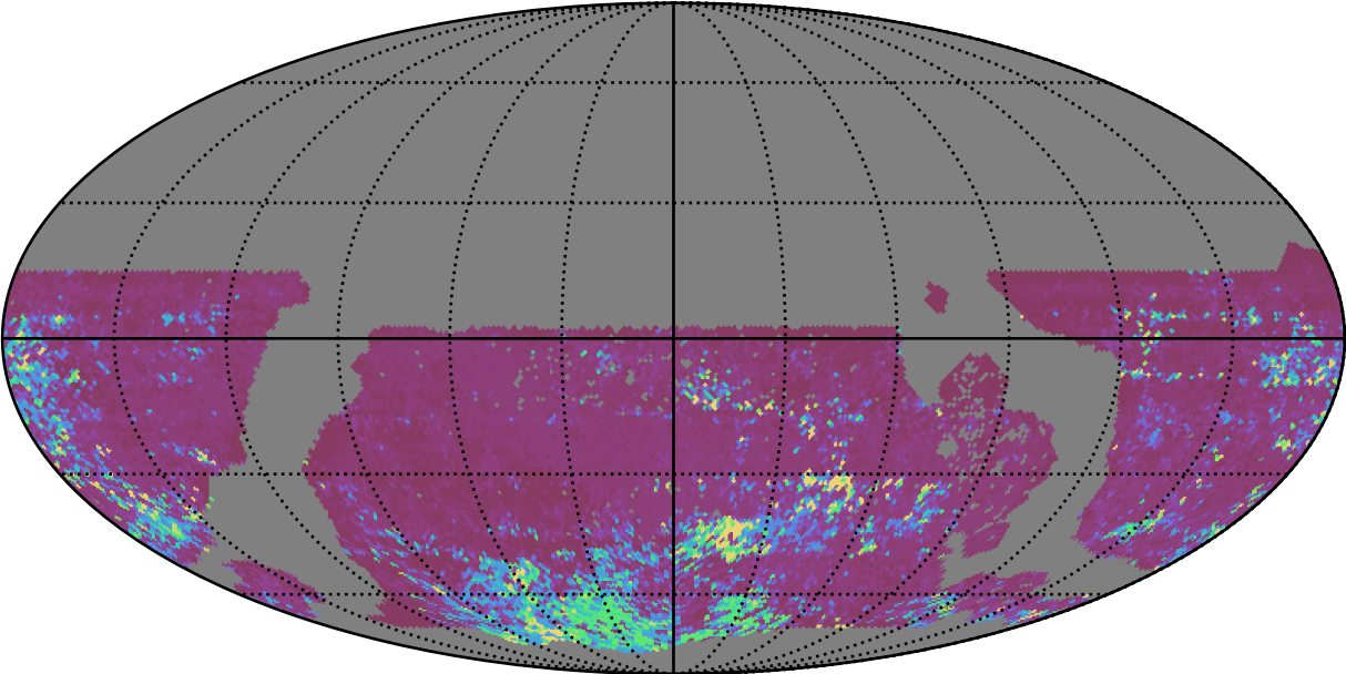
too_elab_r8_d2_giz_v3.4_10yrs WFD z band: 75th Percentile Intranight Timespan
